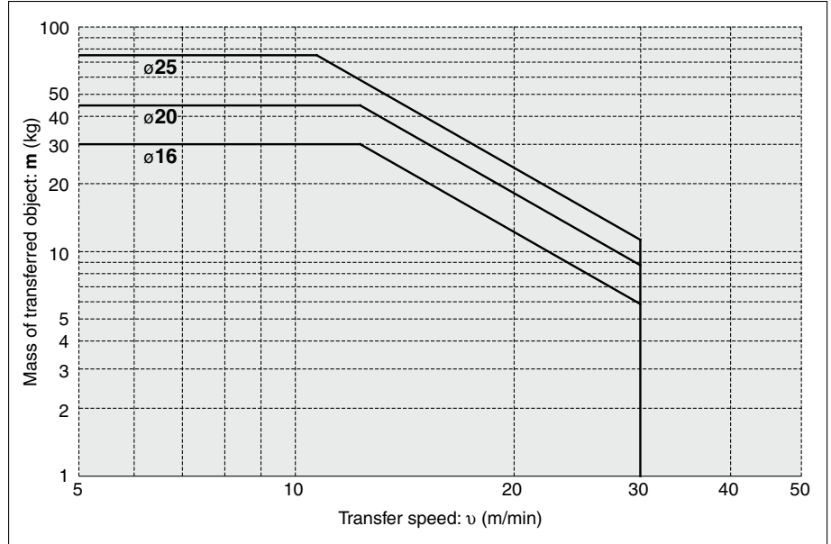
MGPM16 to 25 (Slide Bearing)
